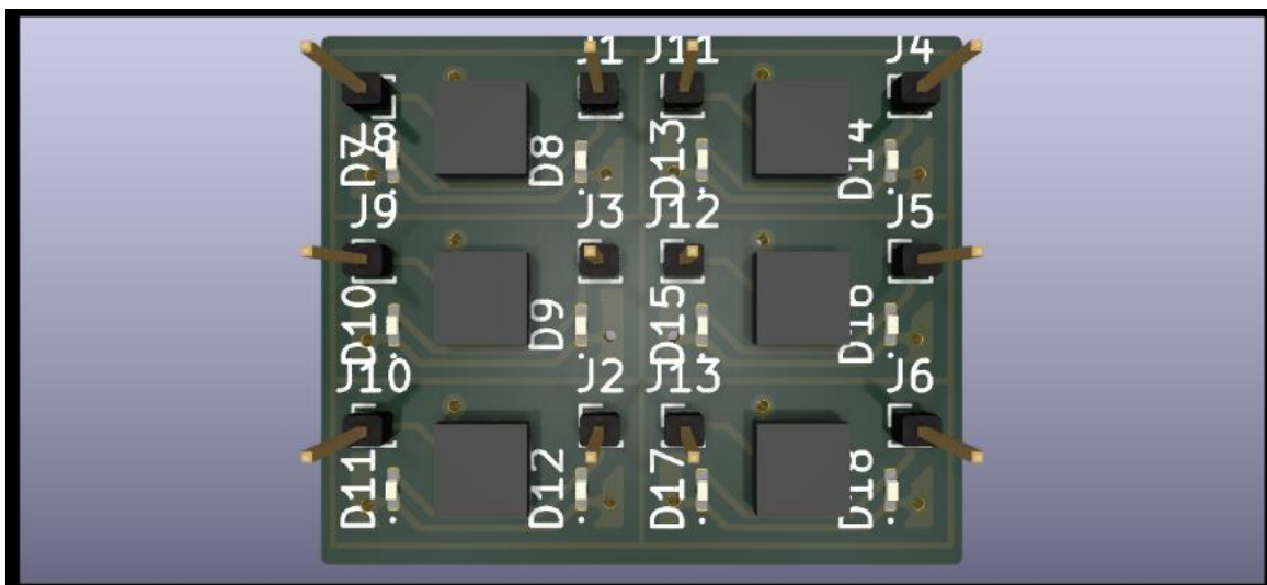
(C) - Sensor Unit
