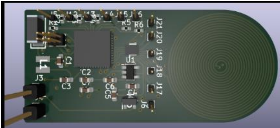
(B) - Control Unit Back
